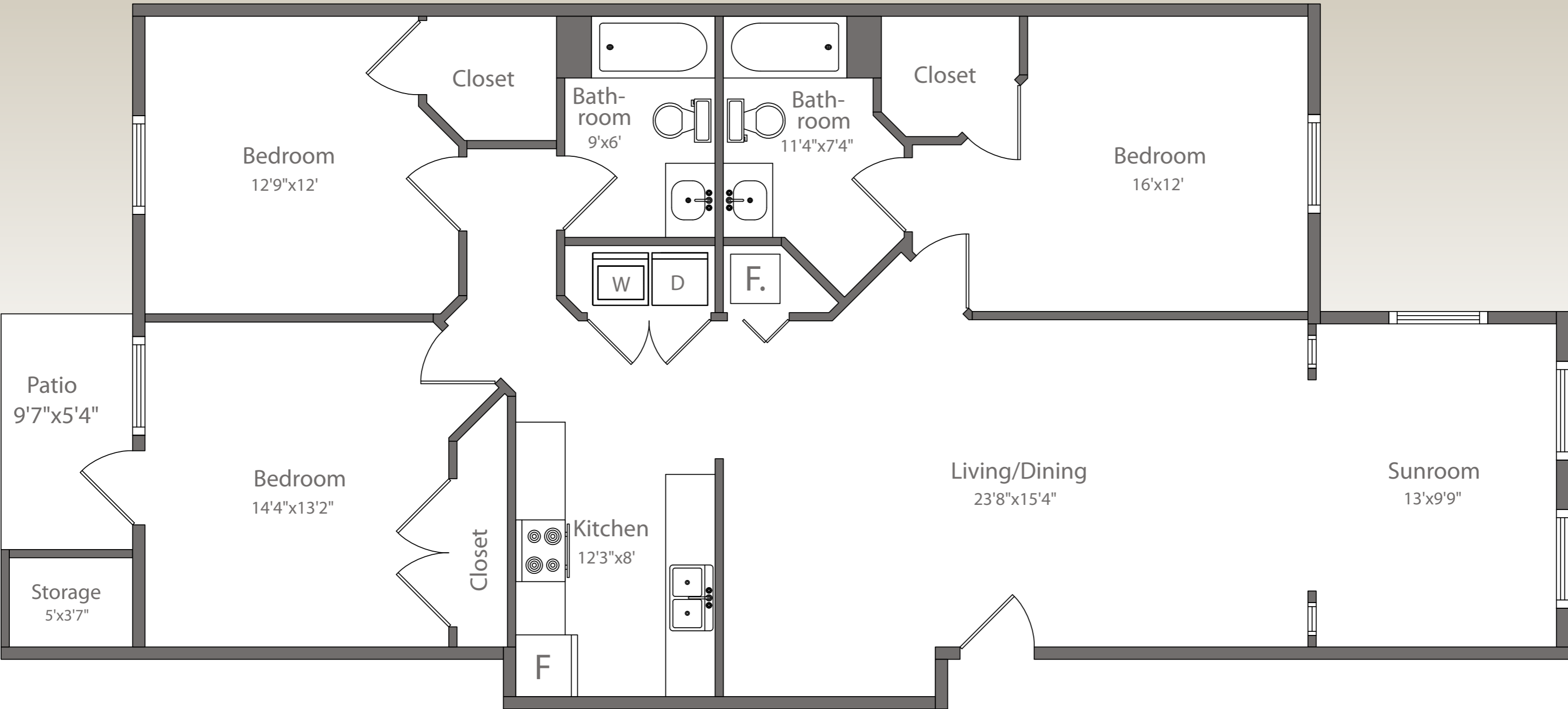
3 Bedroom Unit, with Patio and Sunroom 1475 Square Feet
